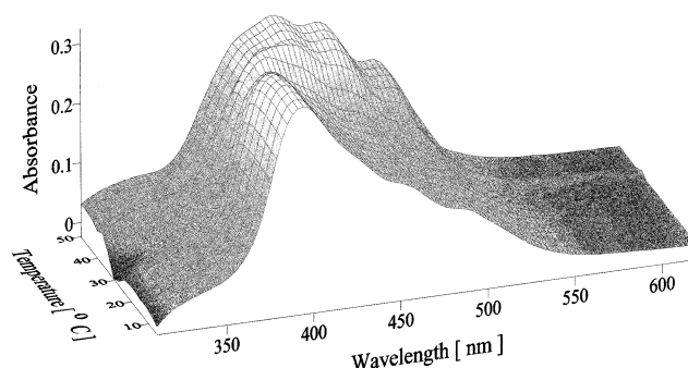
Fig. 4. Temperature dependences of the absorption spectra of zeaxanthin-containing (5 mol%) DPPC liposomes.
